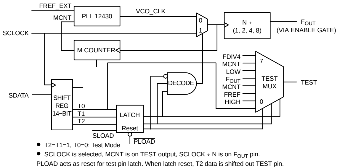
Figure 6. Serial Test Clock Block Diagram
