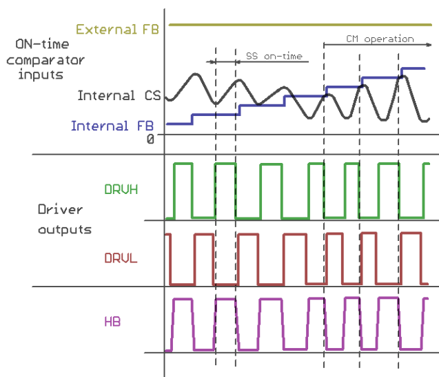
Figure 75. Soft-start Behavior
