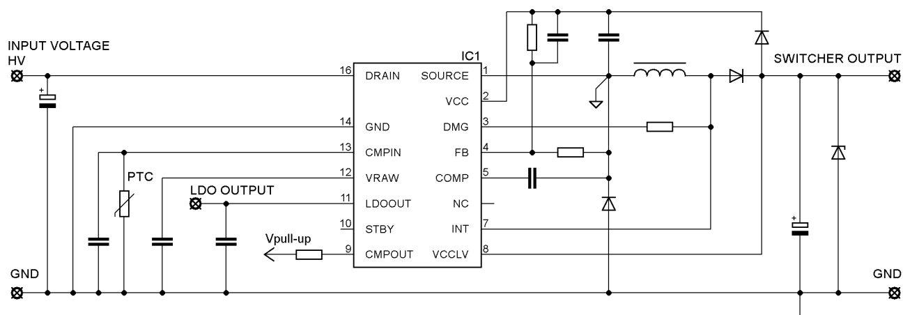
Figure 1. Application Schematic
