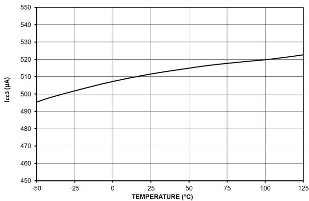
Figure 32. Internal Current Consumption in Skip Mode I CC3
