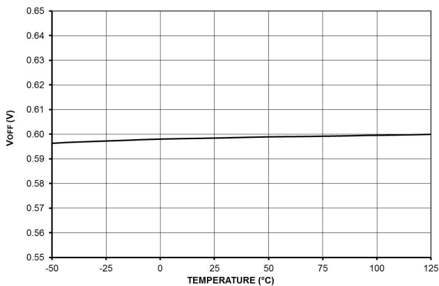
Figure 36. FB Pin Voltage Level Below which is Entered Off Mode V OFF
