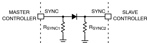
Figure 50. Master-Slave Configuration
