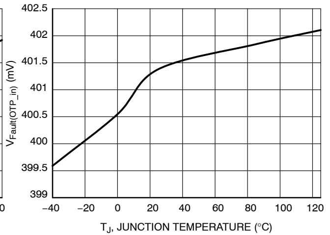
Figure 54. V_{Fault(OTP\_in)} vs. Temperature
