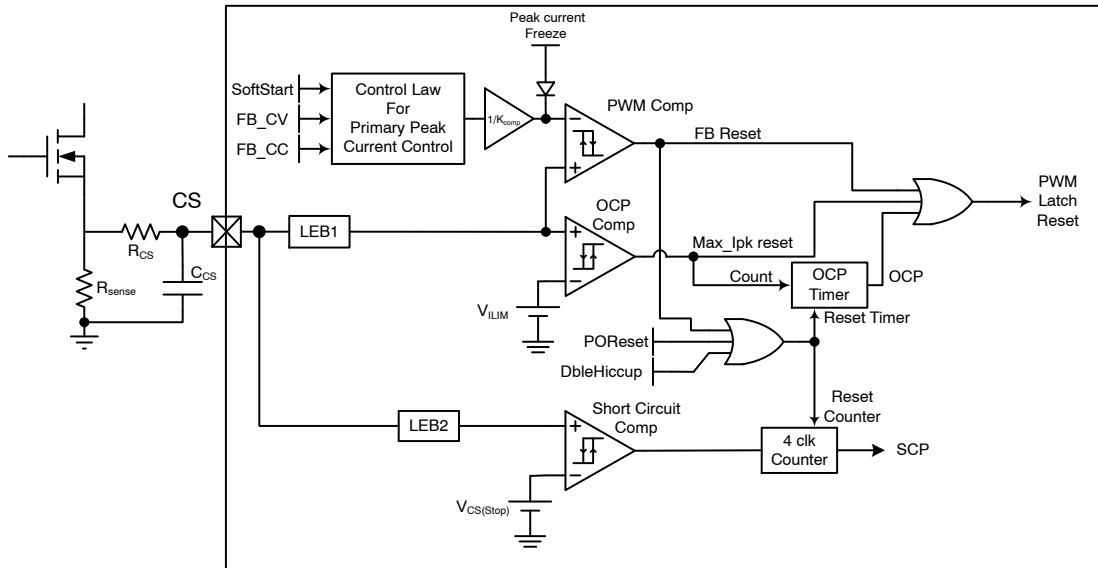
Figure 54. Current Setpoint
