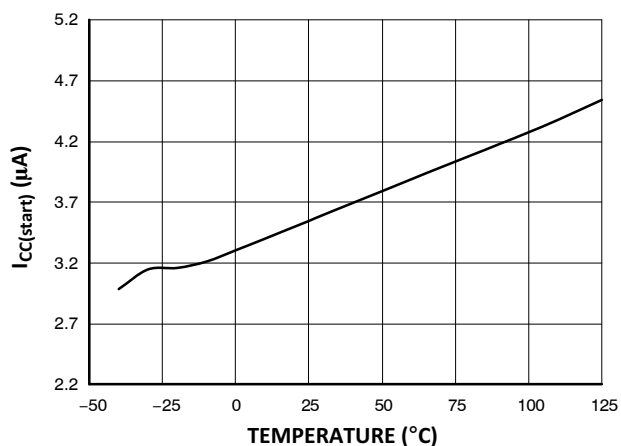
Figure 6. I CC(start) vs. Junction Temperature
