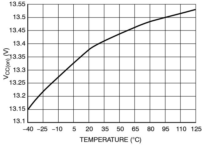
Figure 3. V CC(on)
