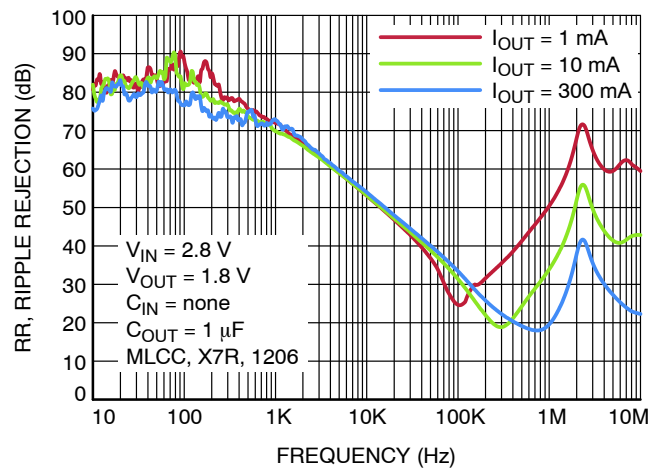
Figure 12. Power Supply Rejection Ratio, C_{OUT} = 1 \mu F
