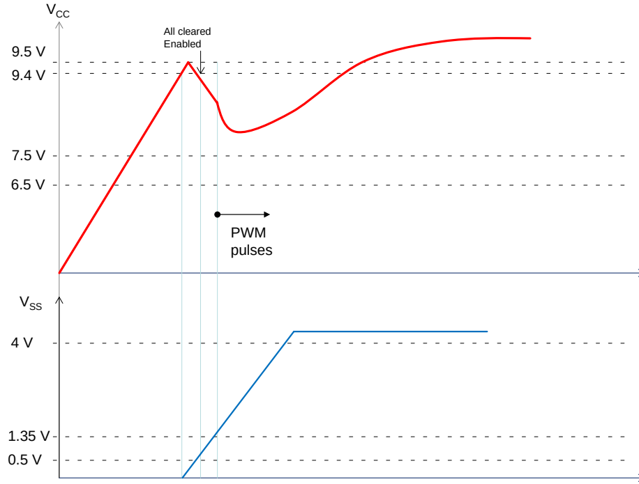
Figure 45. A Typical Startup Sequence in Which the Auxiliary Voltage Builds Up in Time
