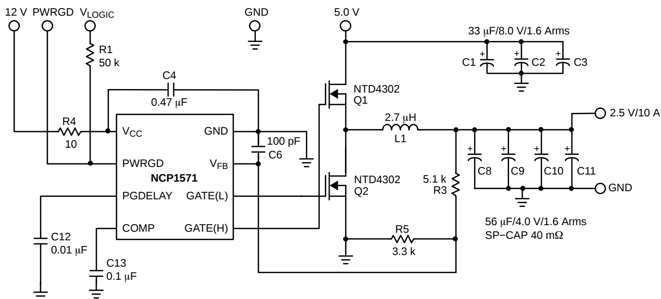
Figure 1. Applications Circuit
