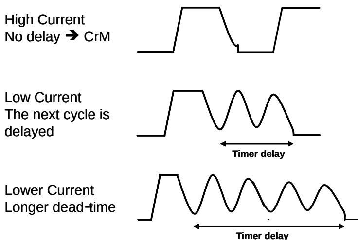
Figure 59. CCFF Operation
