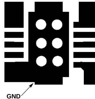
Figure 21. Recommended Footprint
