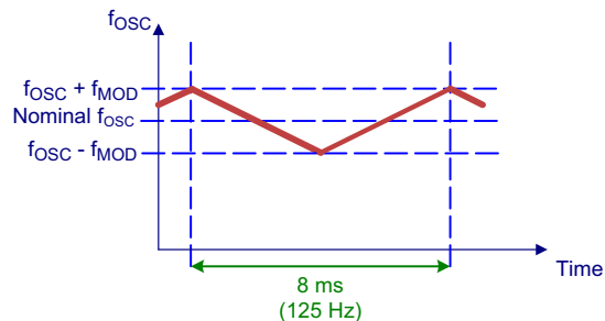
Figure 7. Frequency Jittering
