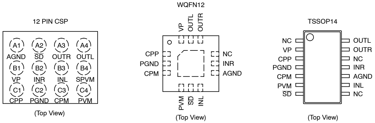
Figure 2. Pin Configurations
