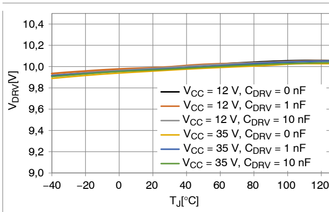
Figure 39. Driver Output Voltage, Ver. xAxxxxx
