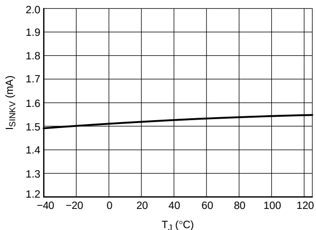
Figure 17. Voltage OTA Current Sink Capability in ECO Mode, V CC = 15 V, V ECODET = 1 V
