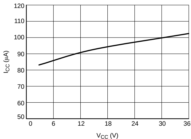
Figure 15. I CC in ECO Mode, T J = 25°C, V ECODET = 1 V, V SNS < V SNSBIAS
