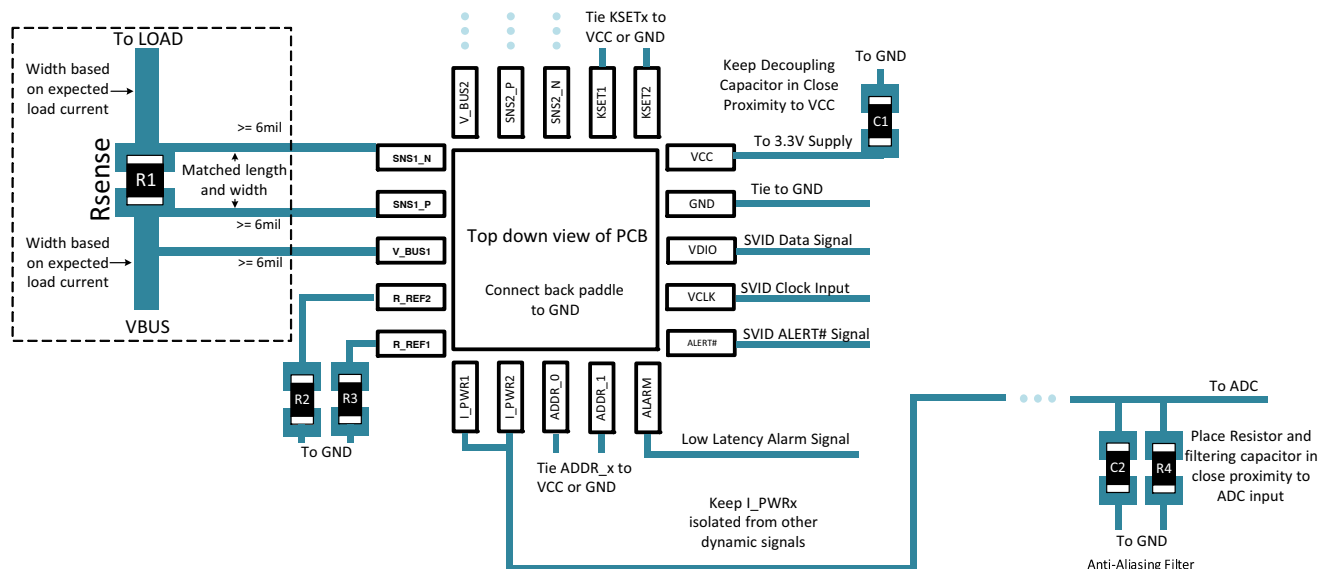
Figure 4. Layout Recommendations
