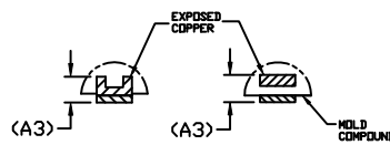
DETAIL B ALTERNATE CONSTRUCTIONS
