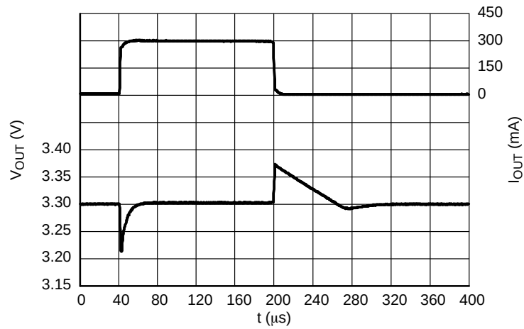
Figure 50. Load Transients, 3.3 V Version, I_{OUT} = 1 - 300 \text{ mA} , t_R = t_F = 0.5 \text{ } \mu\text{s} , V_{IN} = 4.3 \text{ V}
