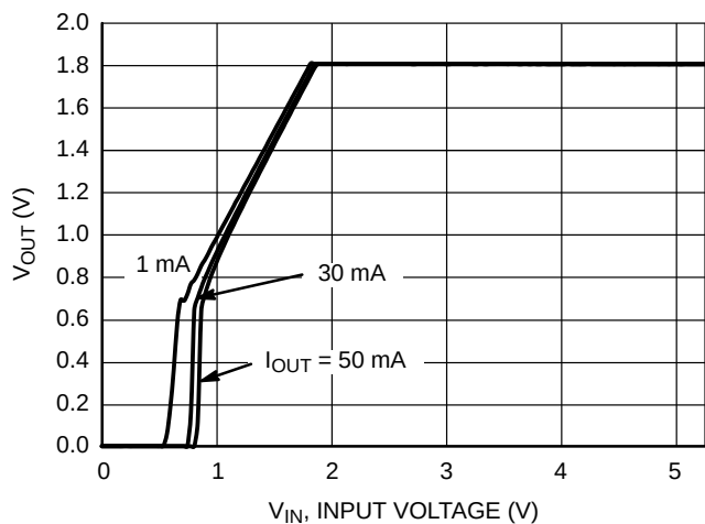
Figure 24. Output Voltage vs. Input Voltage, 1.8 V Version
