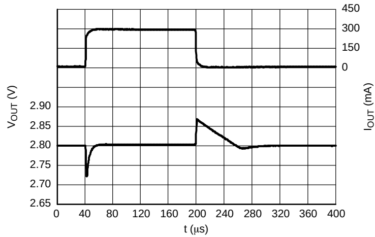
Figure 49. Load Transients, 2.8 V Version, I_{OUT} = 1 - 300 \text{ mA} , t_R = t_F = 0.5 \text{ } \mu\text{s} , V_{IN} = 3.8 \text{ V}
