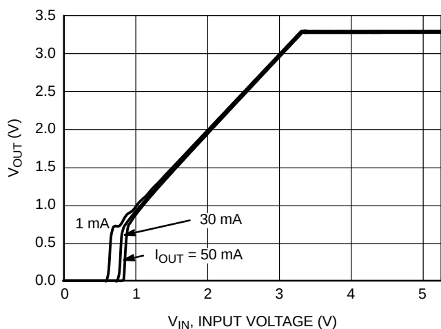
Figure 26. Output Voltage vs. Input Voltage, 3.3 V Version
