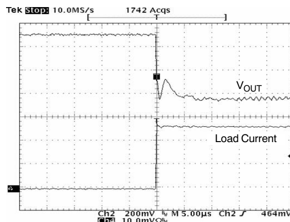
Figure 8. Typical Step Load Response
