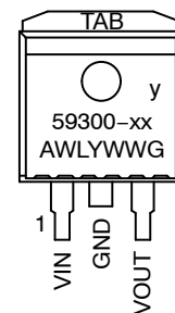
D 2 PAK3
