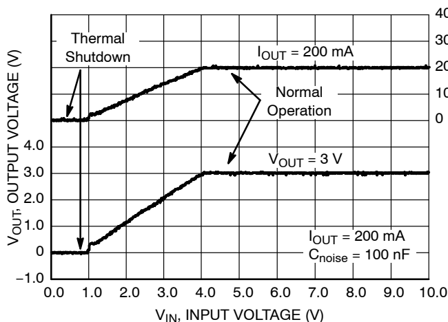
Figure 43. Thermal Shutdown Protection V_{OUT} = 3 V, C_{noise} = 100 nF, C_{OUT} = 1 \mu F
