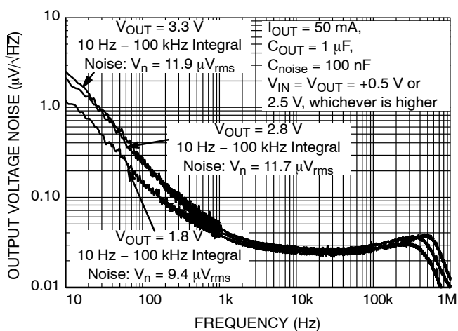
Figure 19. Output Noise vs. Frequency, C_{OUT} = 1 \mu F , C_{noise} = 100 nF , I_{OUT} = 50 mA
