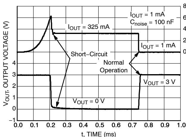
Figure 41. Short-Circuit Protection, V_{OUT} = 3 V, C_{OUT} = 1 \mu F, C_{noise} = 100 nF
