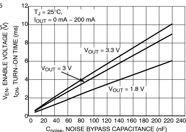
Figure 40. Turn-On Time vs. Noise Bypass Capacitance, C_{OUT} = 1 \mu F, I_{OUT} = 0 mA - 200 mA
