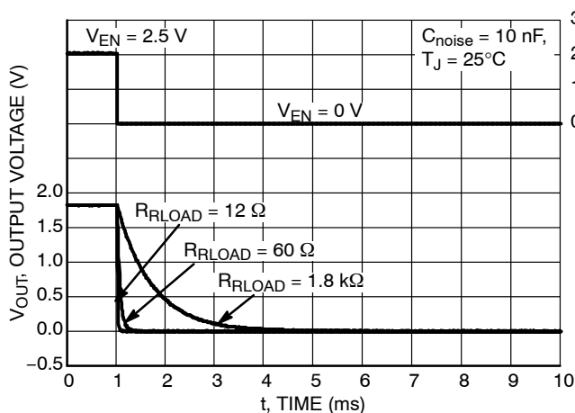
Figure 39. Turn-Off Response V_{OUT} = 1.8 V, C_{OUT} = 1 \mu F
