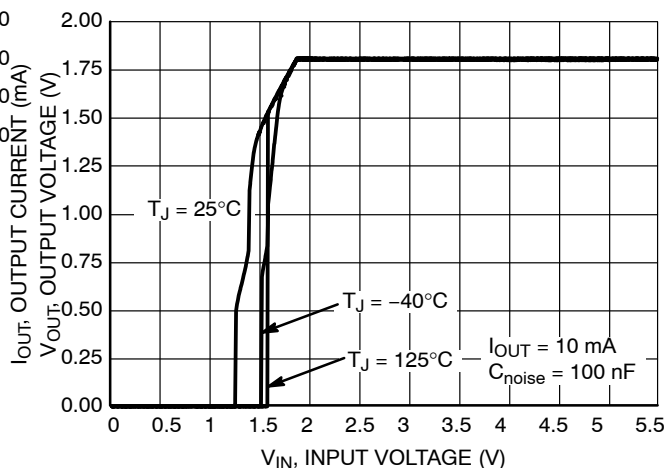
Figure 44. Output Voltage vs. Input Voltage, V_{OUT} = 1.8 V, C_{OUT} = 1 \mu F
