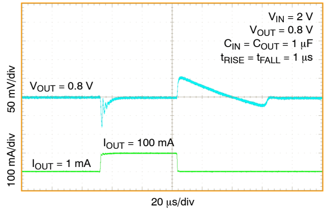
Figure 4. Load Transient Response, 1 mA – 100 mA NCP752A/B, V_{OUT} = 0.8 V
