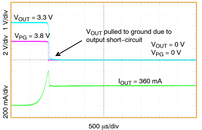
Figure 49. Short-Circuit Response NCP752B, V_{OUT} = 3.3 V
