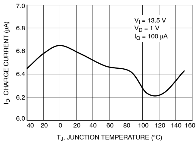
Figure 31. Charge Current vs. Junction Temperature
