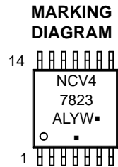
TSSOP-14 Exposed Pad CASE 948AW
