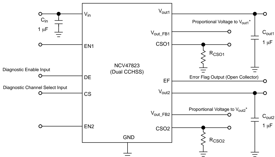
Figure 1. Application Schematic
