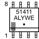
SO-8 D SUFFIX CASE 751
