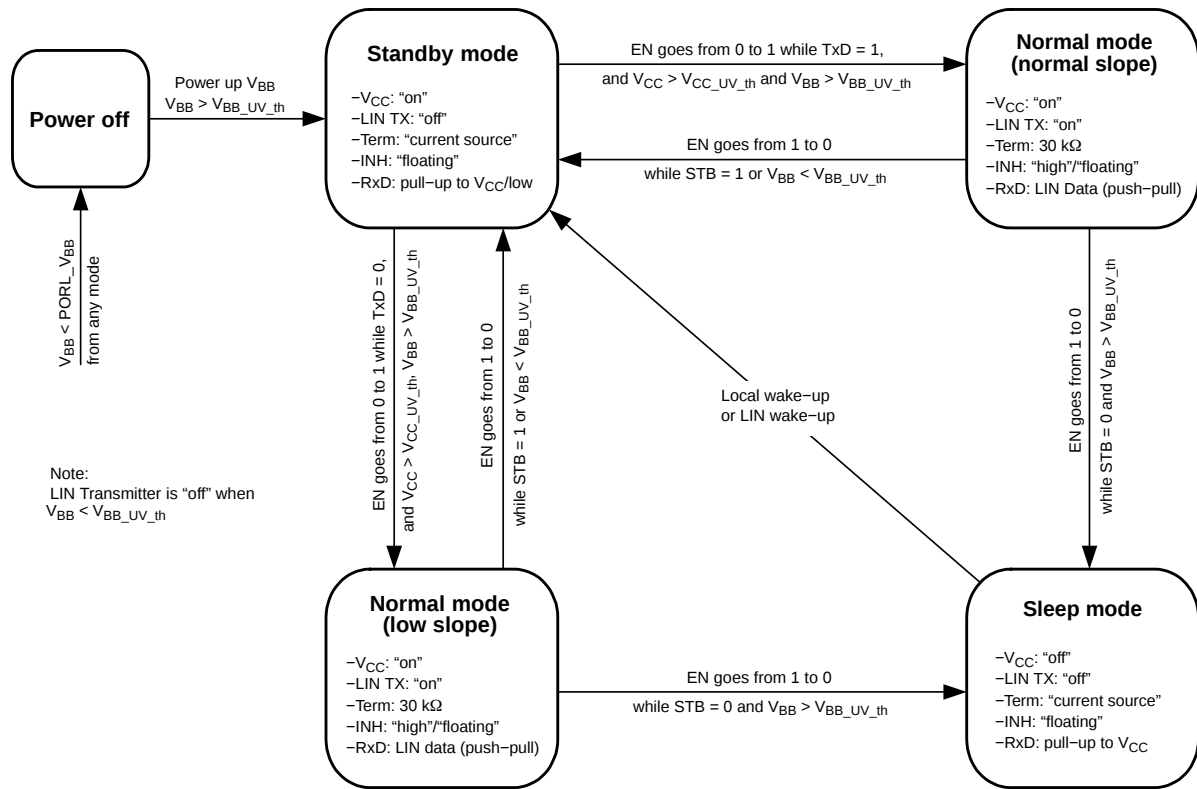
Figure 3. State Diagram
