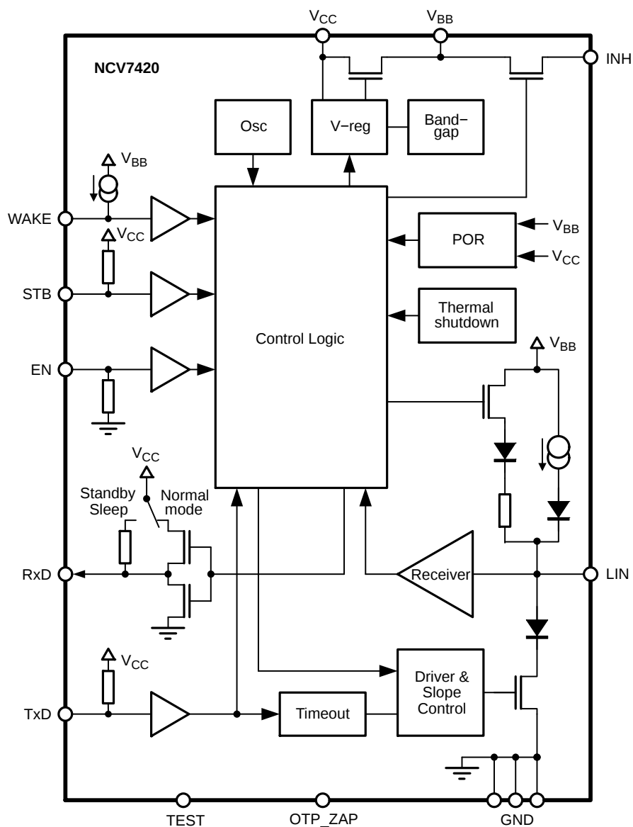
Figure 1. Block Diagram
