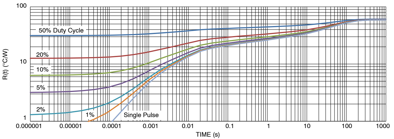
Figure 16. SOIC 28-Lead Thermal Duty Cycle Curve on 986 \text{mm}^2 Spreader Test Board
