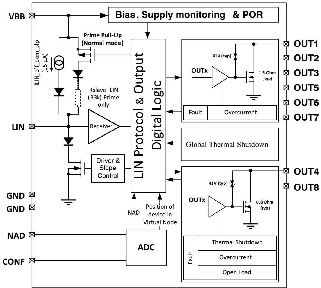
Figure 1. Block Diagram
