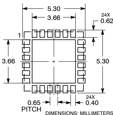
RECOMMENDED SOLDERING FOOTPRINT
