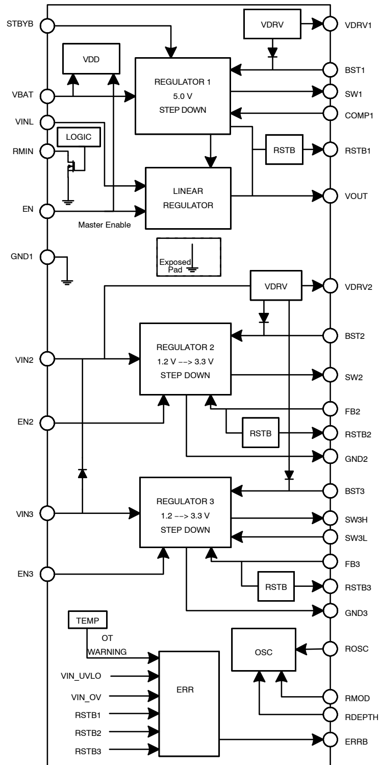
Figure 1. NCV97311A Block Diagram – 5.0 V Version
