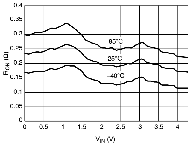
Figure 11. On-Resistance vs. Input Voltage @ V_{CC} = 4.3 V
