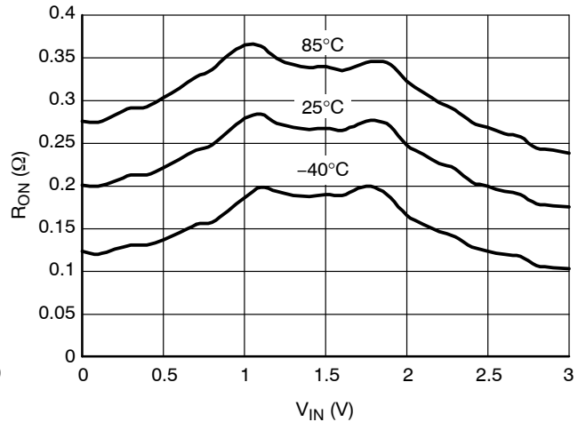
Figure 10. On-Resistance vs. Input Voltage @ V_{CC} = 3.0 V
