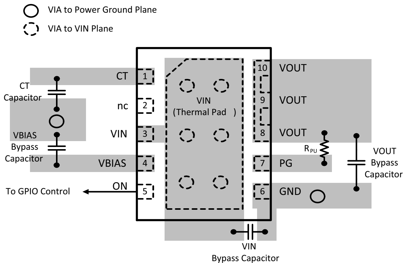
Figure 43. Layout Example
