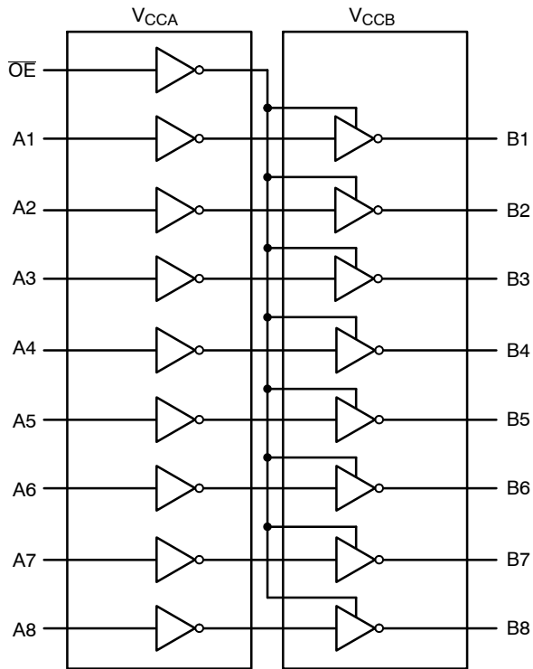
Figure 1. Logic Diagram
