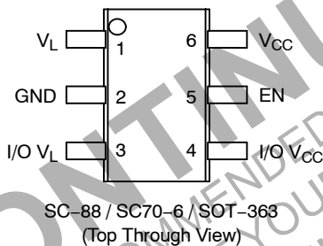
Figure 2. Pinout Diagram
