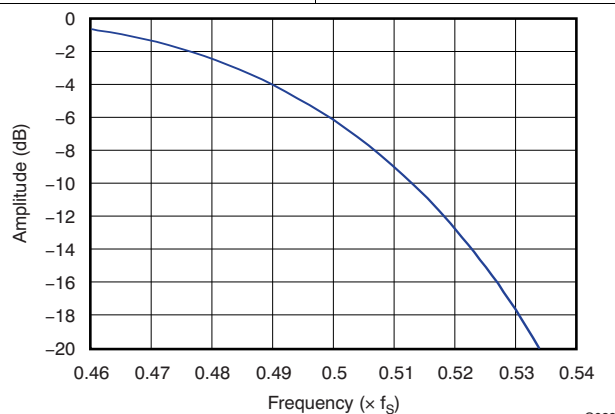
Figure 29. Transition-Band Response
