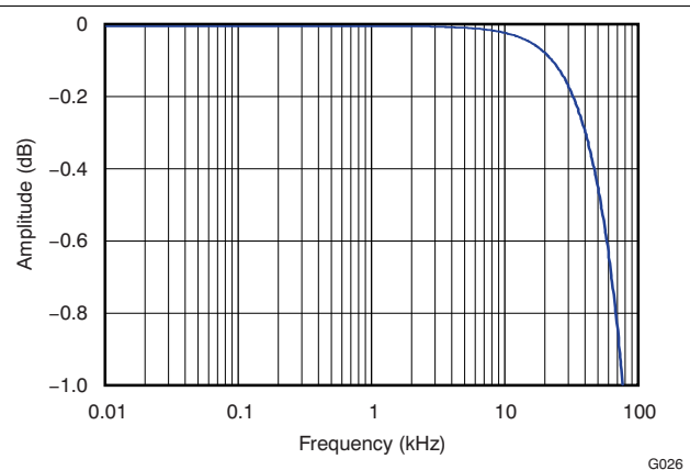
Figure 26. Passband Characteristics
