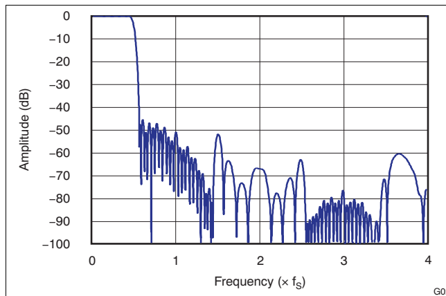
Figure 27. Stop-Band Attenuation
