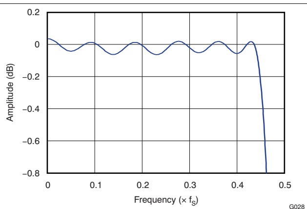
Figure 28. Passband Ripple
