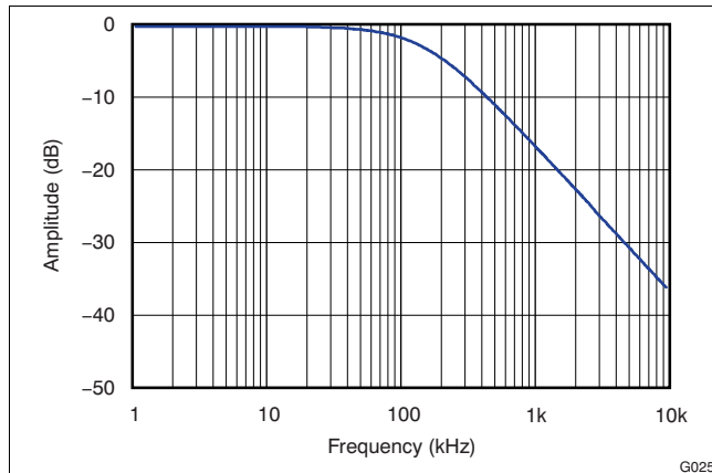
Figure 25. Stop-Band Characteristics
