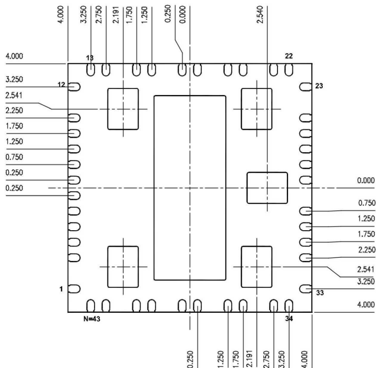
Figure 15. VFQFPN43 8x8mm 43 lead 0.5mm pitch (8x8x1.0 mm) mechanical data 3
