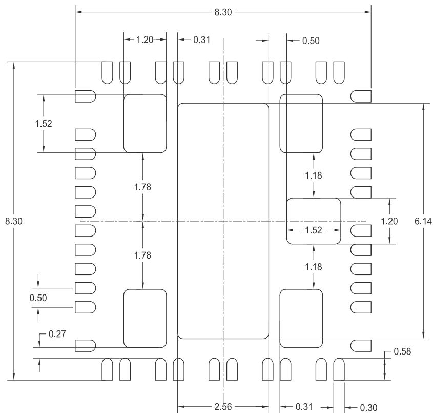
Figure 16. Suggested footprint
