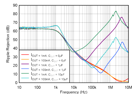
Figure 5-24. PSRR (Ripple Rejection) vs Frequency
