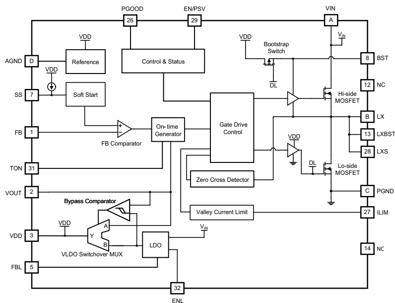
SiC401A/B Functional Block Diagram
