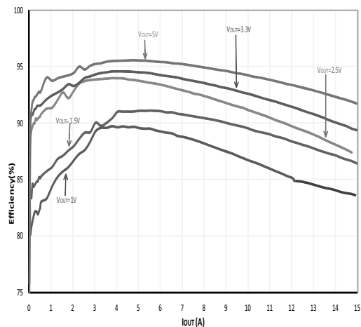
Efficiency Variation with V_{OUT} - P-Save ( V_{DD} = 5V , V_{IN} = 12V , L = 22\mu H (4.6 mΩ) for V_{OUT} = 2.5V, 3.3V and 5V , SiC401B)
