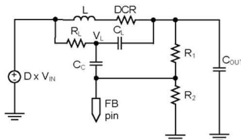
Fig. 13 - Virtual ESR Ramp Circuit
