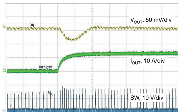
Fig. 32 - Load Step, 0.1 A to 12 A, 1 A/ \mu s, t = 10\text{ }\mu\text{s/div} Forced Continuous Conduction Mode
