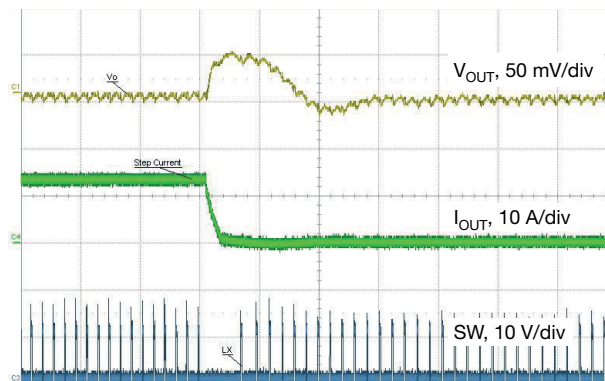
Fig. 35 - Load Release, 12 A to 0.1 A, 1 A/ \mu s, t = 20\text{ }\mu\text{s/div} Forced Continuous Conduction Mode
