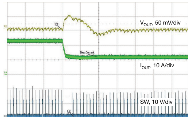
Fig. 33 - Load Release, 24 A to 12 A, 1 A/ \mu s, t = 10\text{ }\mu\text{s/div}
