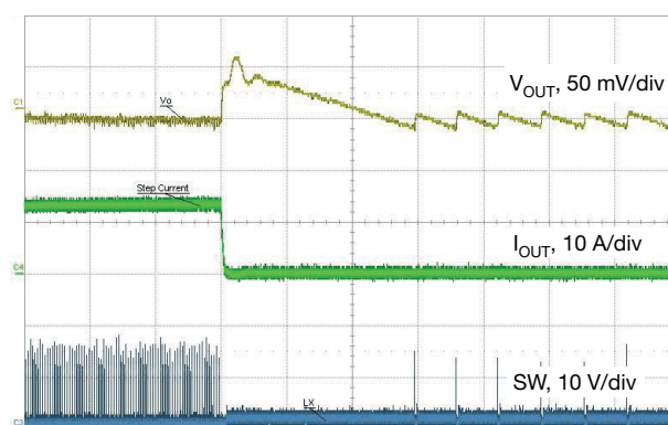
Fig. 34 - Load Release, 12 A to 0.1 A, 1 A/ \mu s, t = 50\text{ }\mu\text{s/div} Skip Mode Enabled
