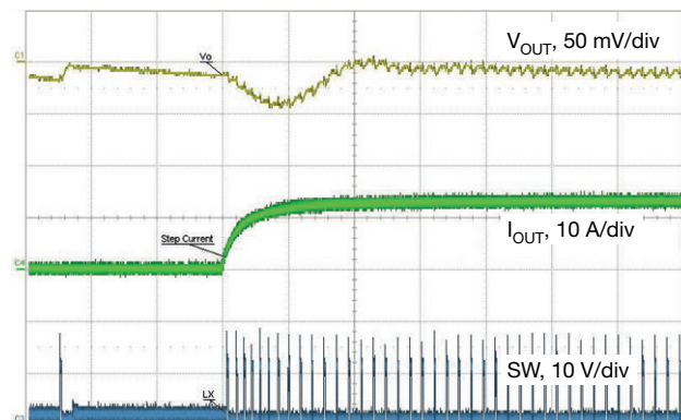
Fig. 31 - Load Step, 0.1 A to 12 A, 1 A/ \mu s, t = 10\text{ }\mu\text{s/div} Skip Mode Enabled
