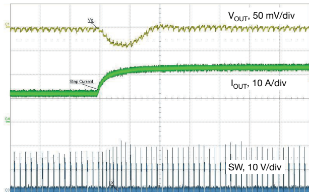
Fig. 30 - Load Step, 12 A to 24 A, 1 A/ \mu s, t = 10\text{ }\mu\text{s/div}
