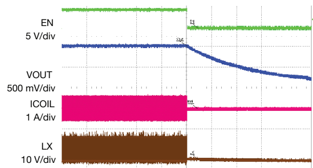
Fig. 14 - Shut-Down, I_{OUT} = 0 A, Time = 200 ms/div
