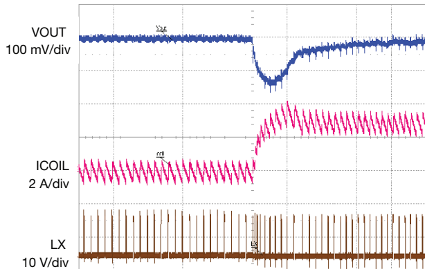
Fig. 10 - Load Step Undershoot Response, I_{OUT} = 0 A to 3 A, Time = 10 \mu s/div
