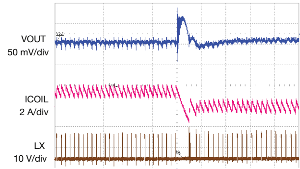
Fig. 12 - Load Step Overshoot Response, I_{OUT} = 1.5 A to 0 A, Time = 10 \mu s/div
