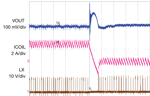
Fig. 13 - Load Step Overshoot Response, I_{OUT} = 3 A to 0 A, Time = 10 \mu s/div
