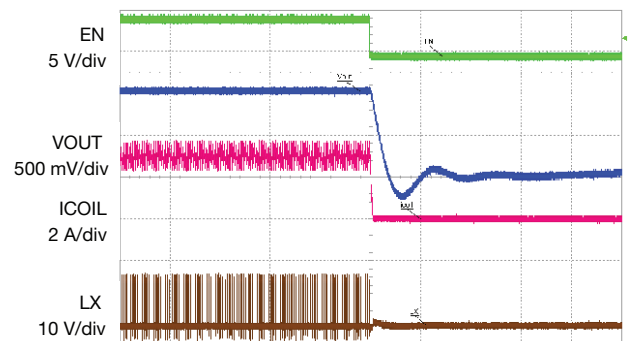
Fig. 17 - Shut-Down, I_{OUT} = 3\text{ A} , Time = 50 \mu\text{s} /div
