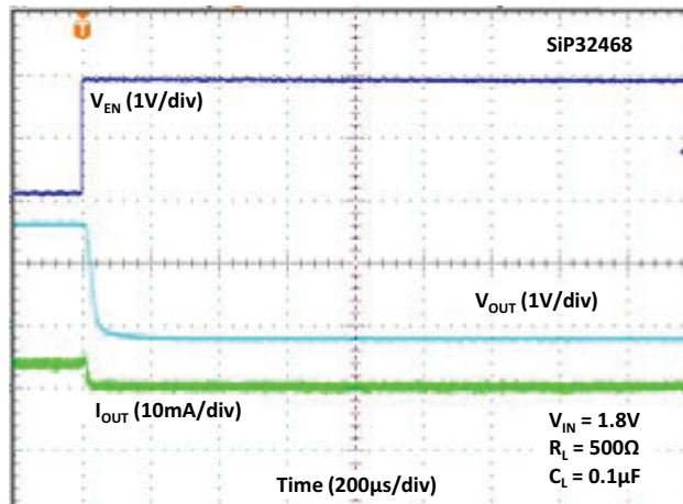
Fig. 33 - Turn-off Time
