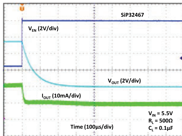
Fig. 31 - Turn-off Time
