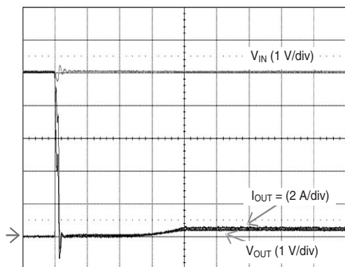
Short Circuit through 0.3 \Omega , V_{in} = 5 \text{ V}
