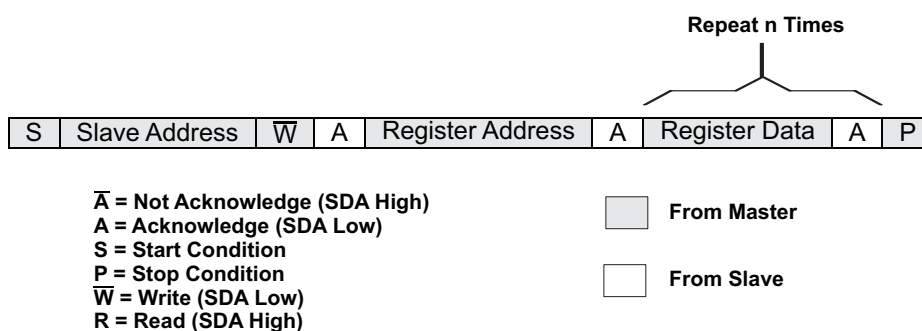
Figure 23. I²C Write Cycle with Register Address and Data
