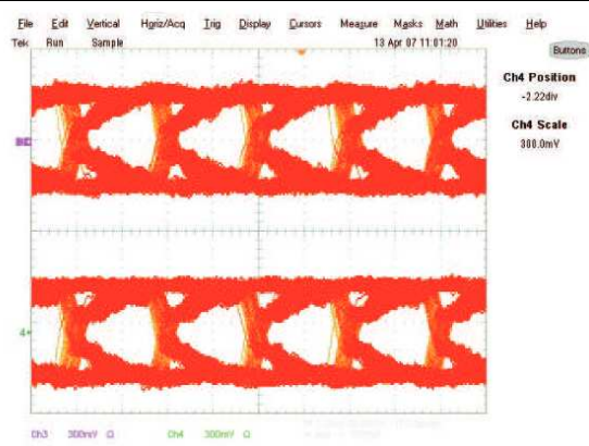
Figure 33. Typical Eye Pattern SN65LVDS051: All Buffers
