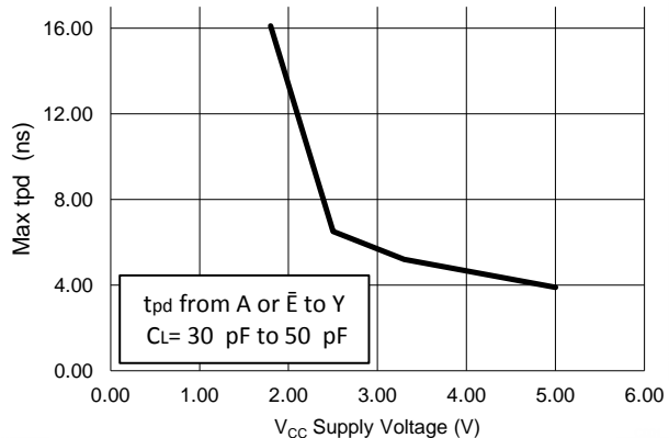
Figure 2. Time Propagation Delay vs V CC , C L = 30 pF or 50 pF
