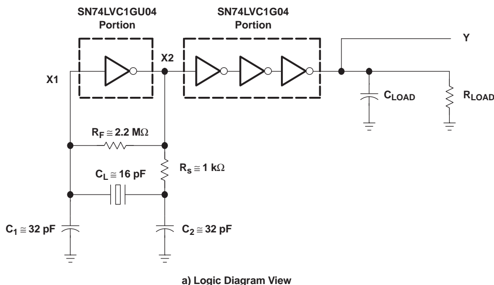
Figure 3. Oscillator Circuit
